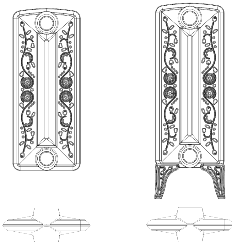
BOHEMIA R 450/225 BOHEMIA R 800/220
