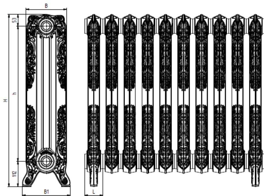
WINDSOR 600/180 s nohou
