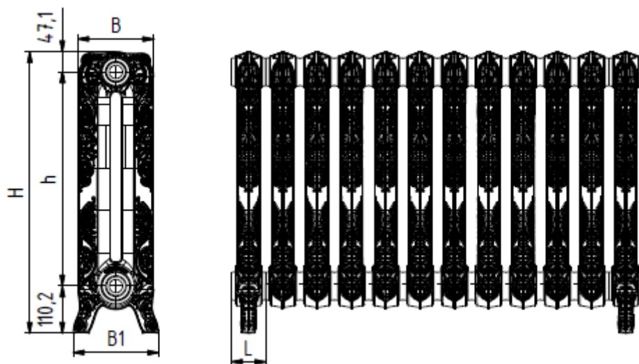
WINDSOR 500/177 s nohou
